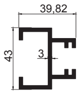
BC-105 K-Ray 1,171 kg/m
