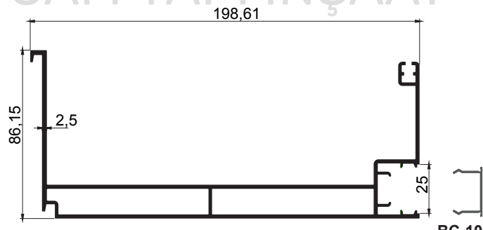
BC-103 Oluk 3,512 kg/m
