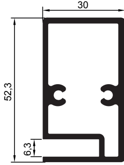
RK-101 Sabit Yatay 1.225 kg/m
