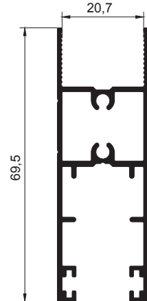
SS-124 ISICAM Alt Baza 0,764 kg/m
