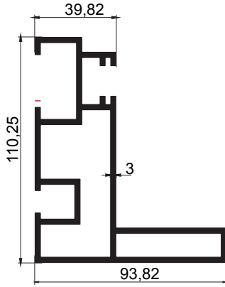
BC-106 B-Ray 3,984 kg/m
