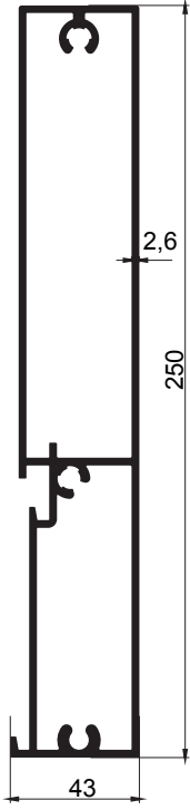
BC-102 Kapatma 4,494 kg/m
